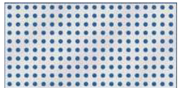
2,50 mm. hole, 19% open area, 5 mm. parallel pitch.
